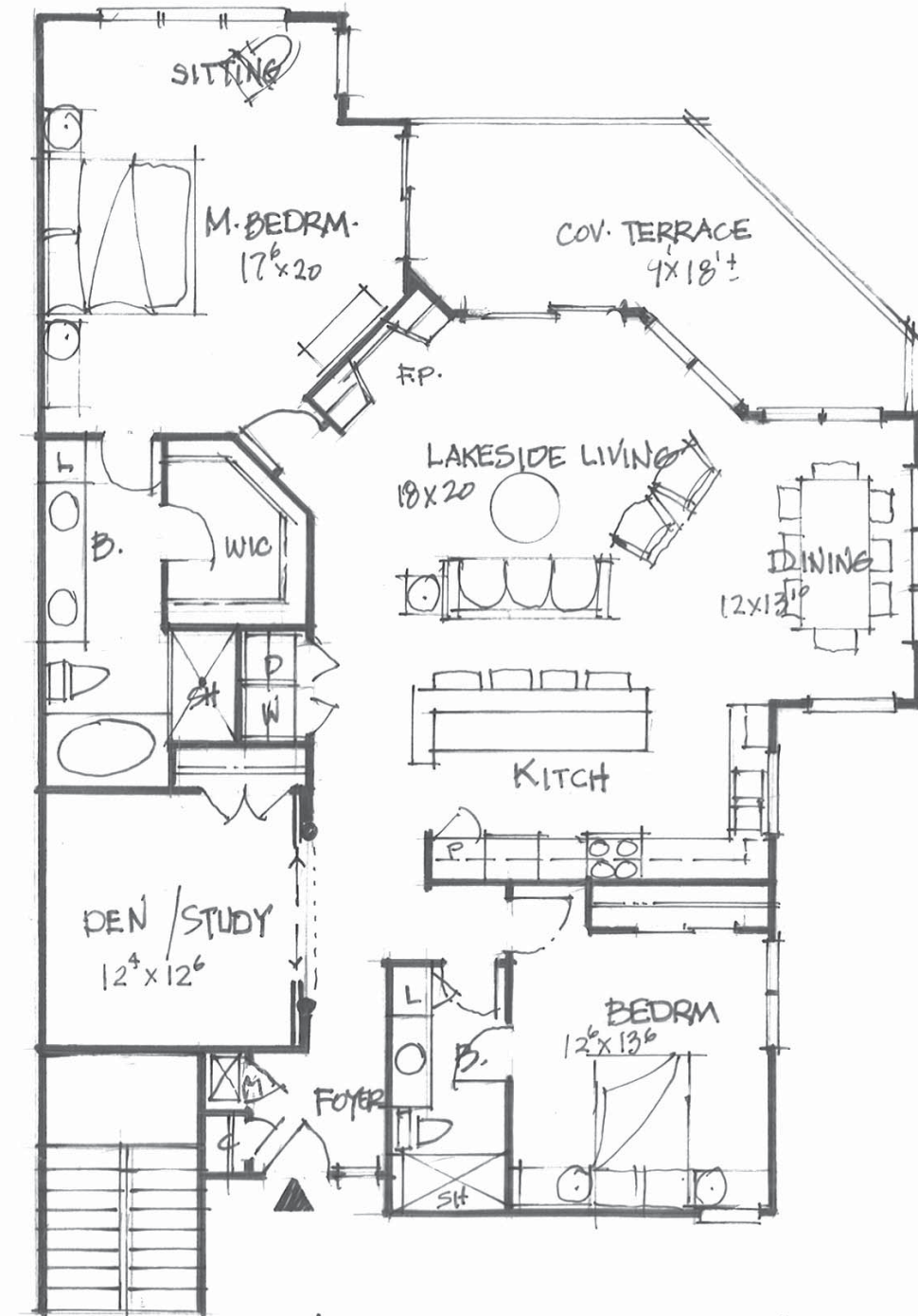
UNIT C - 2 BDRM / DEN 1860 SF 1/8" = 1'-0"
